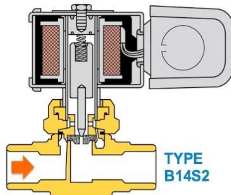
PILOT OPERATED
