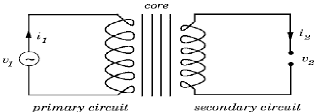
Transformer
