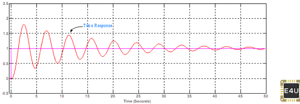
Figure-11: Response of system shown in Figure-10, with K=5.8 , T_d=0.5 , K_i=0.2
