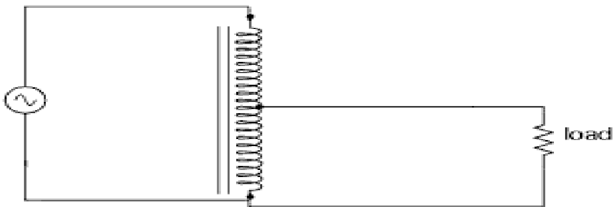
Autotransformer
