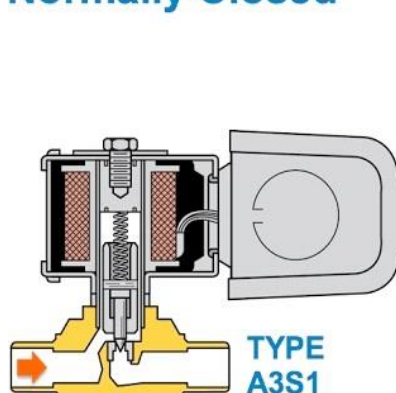
DIRECT ACTING
